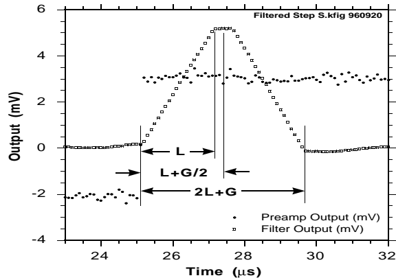
Fig. 1. Trapezoidal finite-impulse response (FIR) energy filter with peaking time L and gap G . The energy value is sampled at the peak of the filter response, that occurs at the time L + \frac{1}{2}G after the event.
