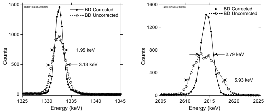
Fig. 2. Accurate ballistic deficit correction calculated by the on-board DSP allows for excellent energy resolution for shaping time as short as t_s = 1\mu\text{s} . Energy values calculated with formula (2.1) (open points) show an inferior energy resolution caused by the rise time variations, that are corrected for when the ballistic deficit correction is applied to the data (full points). Data for ^{60}\text{Co} 1332.5 keV \gamma -line and ^{208}\text{Tl} 2614.5 keV \gamma -line are shown in the left and right panel, respectively.
